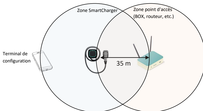
Figure 11 : Zone de couverture WIFI
